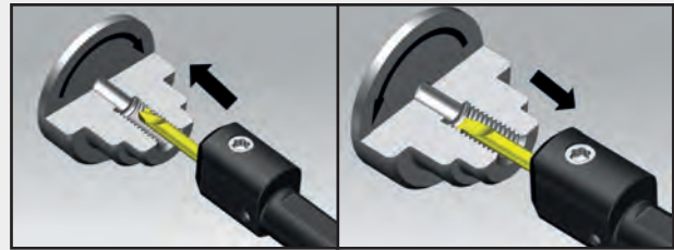
Insert: Left-hand design Direction of rotation: Anticlockwise M4 turning from outside in Insert: Right-hand design Direction of rotation: Clockwise M3 turning from inside out
